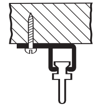
CEILING MOUNT
