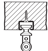
RECESSED MOUNT
