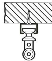
CEILING MOUNT
