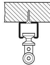
CEILING MOUNT RECESSED MOUNT
