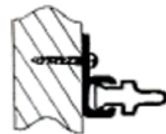
3110/3294 Wall Mount
